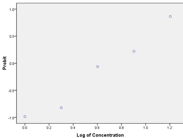
Fig 2: Probit transformed responses diagram of toxicity of Viola odorata extract on the Agonoscena pistaciae (Hemiptera: Psyllidea).
